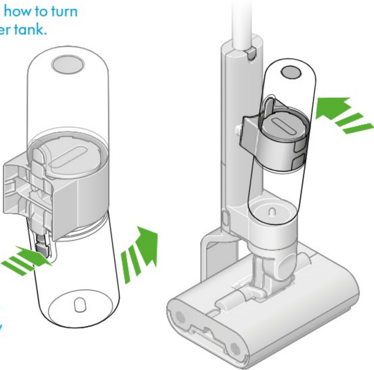
Diagram showing how to reassemble the Dirty water tank.
